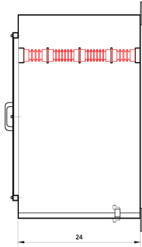
SIDE SECTION-THROUGH
