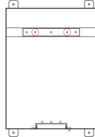
FRONT SECTION-THROUGH
