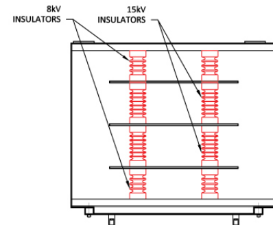
TOP SECTION-THROUGH
